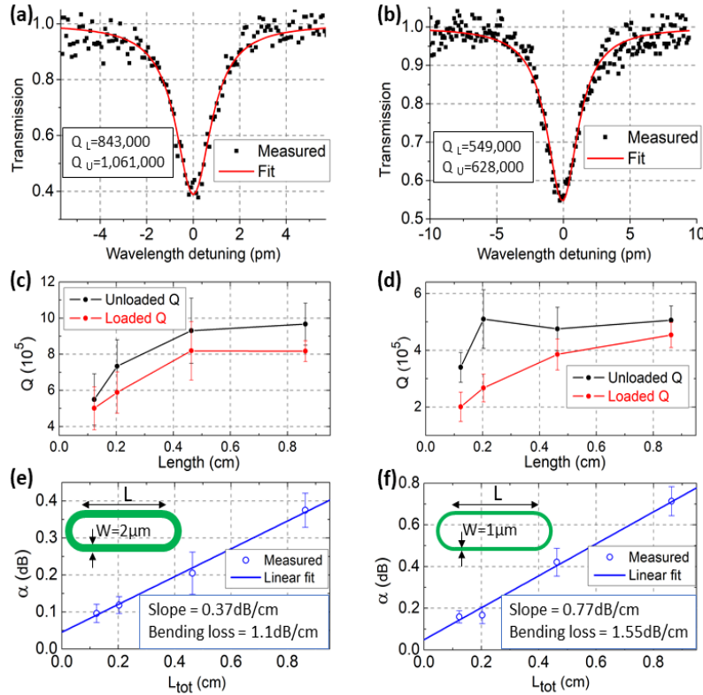
Fig. 4. (a) and (b): Measured (black dots) and fitted (red curves) transmission of RT resonator ( L = 4000 \mu\text{m} ) with W = 2 \mu\text{m} and W = 1 \mu\text{m} , respectively. (c) and (d): Loaded and unloaded Q factors in RT resonator as a function of the total length ( L_{\text{tot}} = 2\pi R + 2L ) for 2 \mu\text{m} and 1 \mu\text{m} wide straight waveguides respectively. (e) and (f): Intrinsic loss in RT resonator as a function of the total length. Average propagation losses of 0.37 \text{ dB/cm} and 0.77 \text{ dB/cm} for 2 \mu\text{m} and 1 \mu\text{m} wide straight waveguides were extracted by linearly fitting the experimental data. The variations in the value of the average propagation losses are set equal to one standard deviation of the losses extracted from several resonances around 1550 \text{ nm} .
