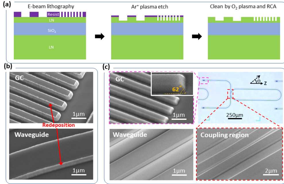
Fig. 3. (a) Fabrication flow of LNOI photonic devices. The LNOI wafer was purchased from NGK Insulators, LTD. (b) SEM pictures of GC and waveguide before RCA cleaning. The redeposition of LN along the sidewalls of the patterned features is clearly visible. (c) Microscope picture of one of the fabricated RT resonators (upper right) and SEM pictures of various photonic components after RCA cleaning. Inset: the sidewall slant angle is 62° from horizontal. The waveguide is 2 μm wide and the coupling region (lower right) between the waveguides features a gap of 200 nm. The sidewall is very smooth after RCA cleaning. \theta is the angle between the propagation direction of the straight waveguide and the crystalline z-axis ( \theta = 0^\circ for the RT shown in the microscope picture).
