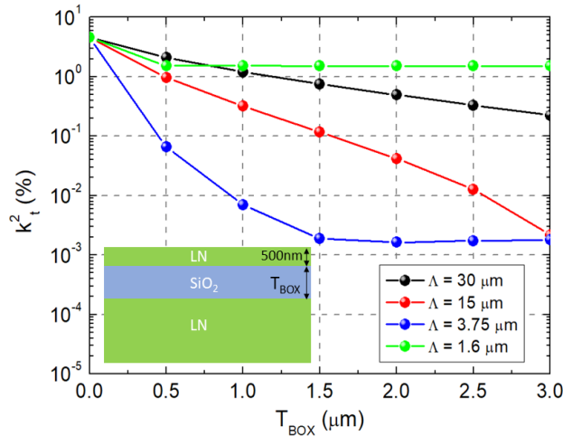
Fig. 1. Simulated electromechanical coupling coefficient ( k_t^2 ) for various T_{\text{BOX}} and acoustic wavelengths ( \Lambda ) on a YZ cut LNOI (see inset for wafer stack). The presence of oxide clearly has a deleterious impact on the device k_t^2 . It is interesting to note how the impact changes with the specific wavelength. This is due to changes in penetration of the acoustic and electric fields in the thin films of LN, oxide and the thick LN substrate. At larger acoustic wavelengths, the oxide thickness is a small fraction of the active SAW devices. At intermediate wavelengths, the oxide becomes a dominant part of the active SAW and its impact on k_t^2 is more dramatic. At the smallest wavelength, the acoustic and electric fields are almost entirely confined in the thin film of LN and the oxide has a lower impact on k_t^2 .
